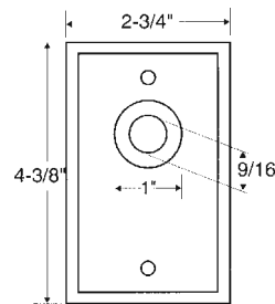
CM9080 Overall Dimension
