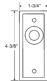
CM9180 Cut Out
