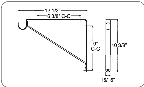
2810 - Shelf and Rod Support
