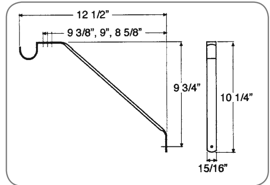
2815 - Fixed Shelf Support
