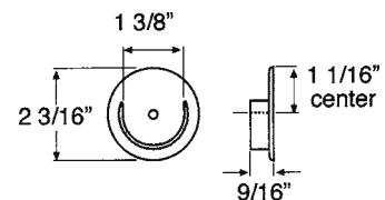
2830 - Pole Socket
