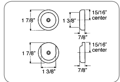
2830 - Pole Socket
