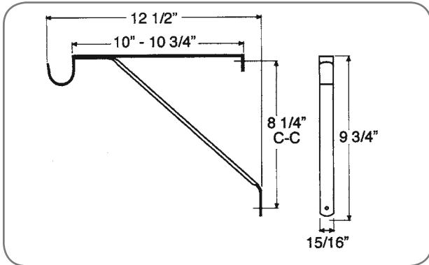
2800 - Shelf and Rod Support
