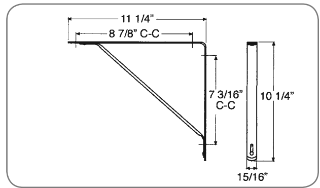
2815 - Fixed Shelf Support
