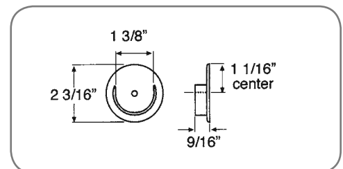
2830 - Pole Socket
