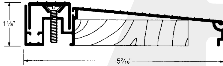
ADJUSTABLE SILL
