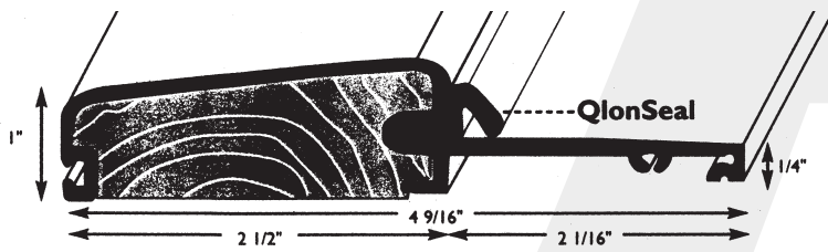
OUTSWING SILL
