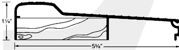
FIXED SILL
